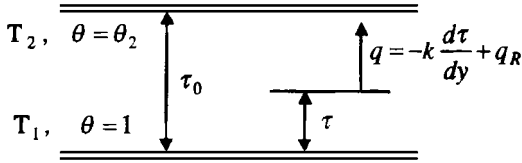
Figure 24.3.1 One-dimensional combined conduction and radiation.
