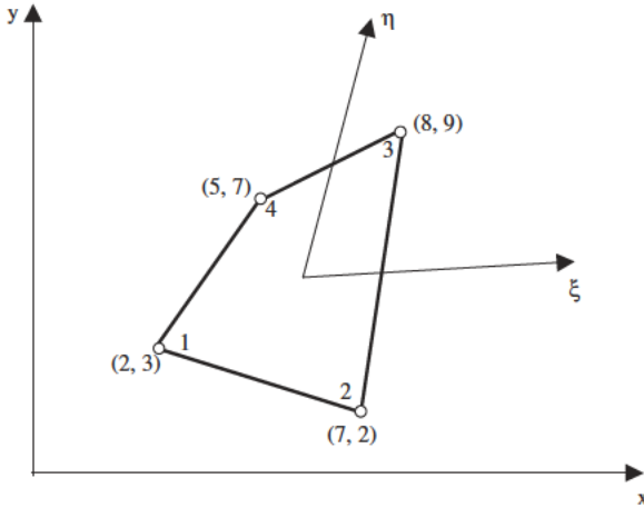
Figure E9.3.2 Geometry for Example 9.3.2.
