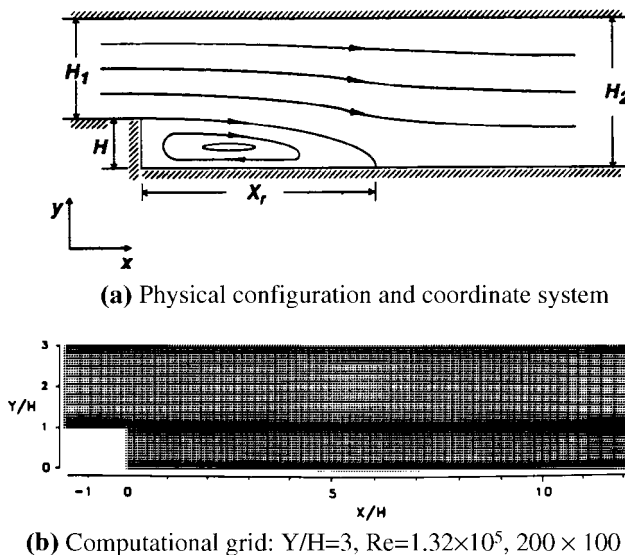
Figure 21.7.1.1 Incompressible turbulent flow backward facing step, 2-D geometry for K - \epsilon model analysis, C_{\mu} = 0.09 , C_{\epsilon 1} = 1.44 , C_{\epsilon 2} = 1.92 , \sigma_k = 1.92 , \sigma_{\epsilon} = 1.0 , CD = 1.68 [Thangam and Speziale, 1988].
