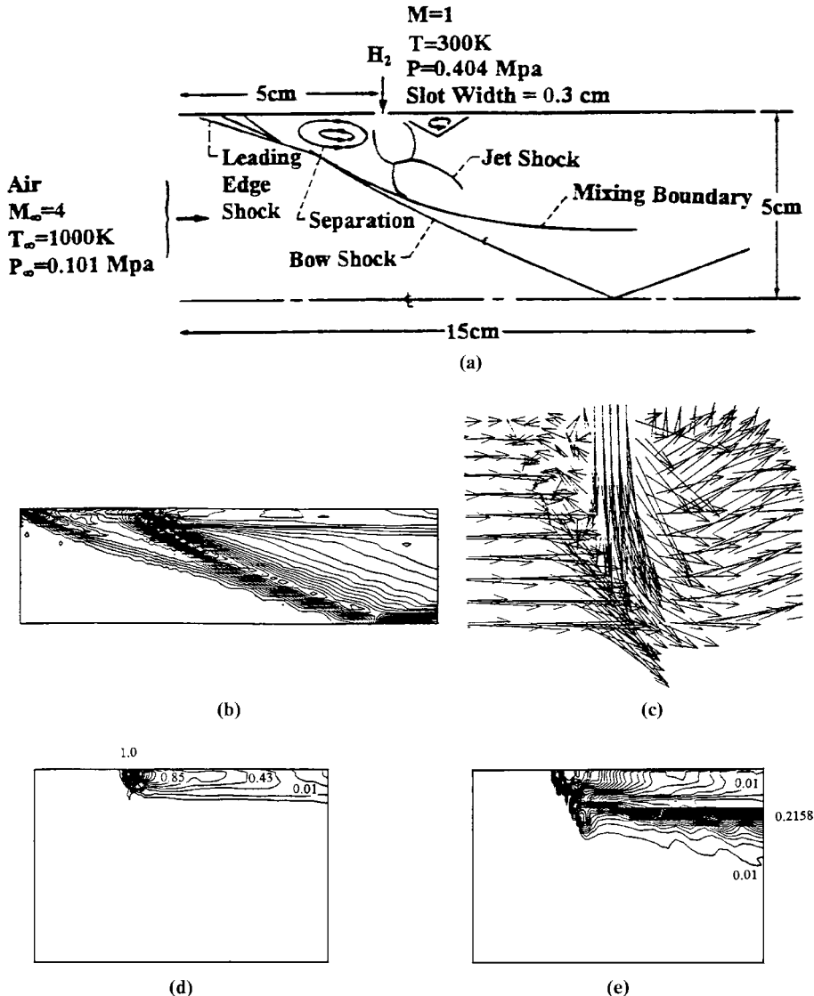
Figure 22.6.2.3 Transverse hydrogen jet injection combustor analysis with K-\epsilon model [Moon, 1998]. (a) Schematics of injection slot, M=1 , T=300 K, P=0.404 Mpa. (b) Pressure contours. (c) Velocity field near the injector. (d) H 2 mass fraction (max = 1.0 min = 0.0, \Delta = 0.01 ). (e) H 2 O mass fraction (max = 0.2158, min = 0.0, \Delta = 0.08 ).
