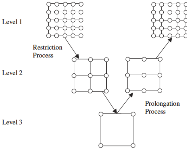
Figure 20.2.1 Three-level multigrid discretization.
