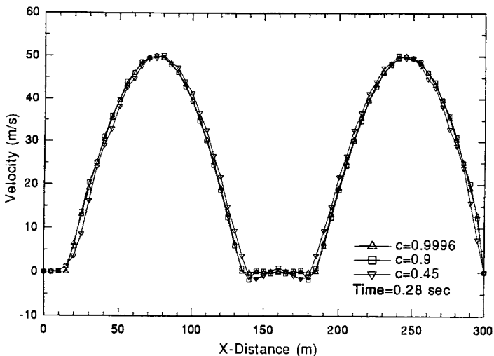
Figure 4.7.4.1 Solution of second order wave equation by midpoint leapfrog scheme, 60 nodes.
