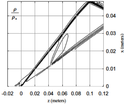
Figure 6.8.2.4 Inviscid fin shock interaction.
