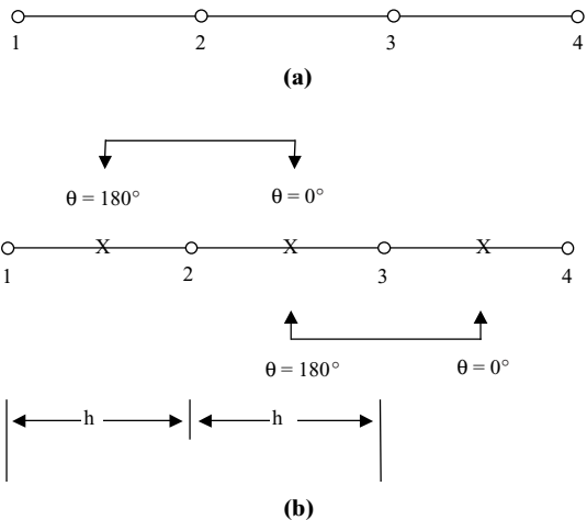
Figure 1.6.1 Example problem, Dirichlet and Neumann boundary conditions. (a) Three elements, four nodes for FDM and FEM. (b) Direction cosines at control surfaces as a result of integration by parts for FVM.
