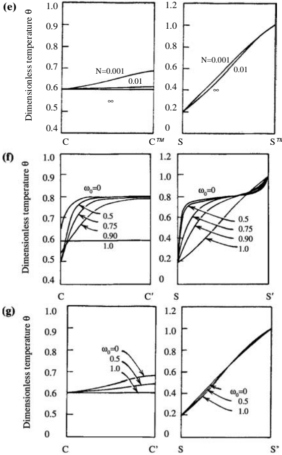
Figure 24.4.5.1 (continued.) (e) Effects of N on the temperature profiles along \overline{CC'} and \overline{SS'} . \tau_0 = 0.1 ; \omega_0 = 0 ; \text{Re Pr} = 100 . (f) Effects of albedo \omega_0 on the temperature profiles along \overline{CC'} and \overline{SS'} . \tau_0 = 1.0 ; N = 0.00 ; \text{Re Pr} = 100 . (g) Effects of albedo \omega_0 on the temperature profiles along \overline{CC'} and \overline{SS'} . \tau_0 = 0.1 ; N = 0.00 ; \text{Re Pr} = 100 .
