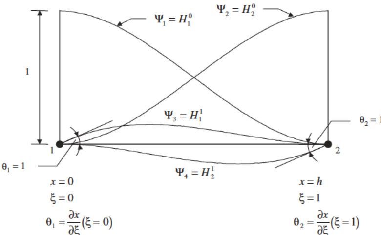
Figure 17.1.2 Hermite polynomial.
