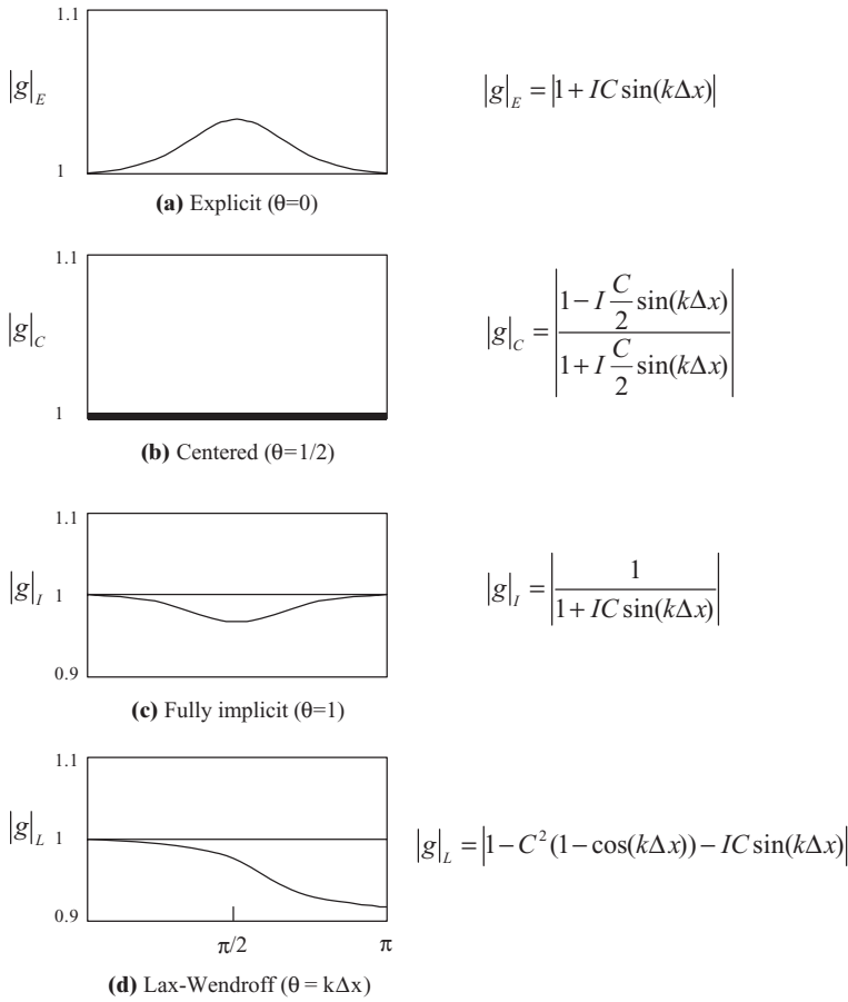
Figure 4.5.3 Amplification factors.
