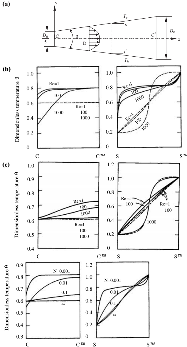
Figure 24.4.5.1 Two-dimensional analysis with three-dimensional heat flux formulation in combined conduction, convection, and radiation. (a) Geometry of two-dimensional radiation problem. (b) Effects of Reynolds number on the temperature profiles along \overline{CC'} and \overline{SS'} . \tau_0 = 1.0 ; Pr = 1.0 . (—) \omega_0 = 0 ; (---) \omega_0 = 1 . (c) Effects of Reynolds number on the temperature profiles along \overline{CC'} and \overline{SS'} . \tau_0 = 0.1 ; N = 0.001 ; Pr = 1.0 . (—) \omega_0 = 0 ; (---) \omega_0 = 1 . (d) Effects of N on the temperature profiles along \overline{CC'} and \overline{SS'} . \tau_0 = 0.1 ; \omega_0 = 0 ; Re Pr = 100 .
