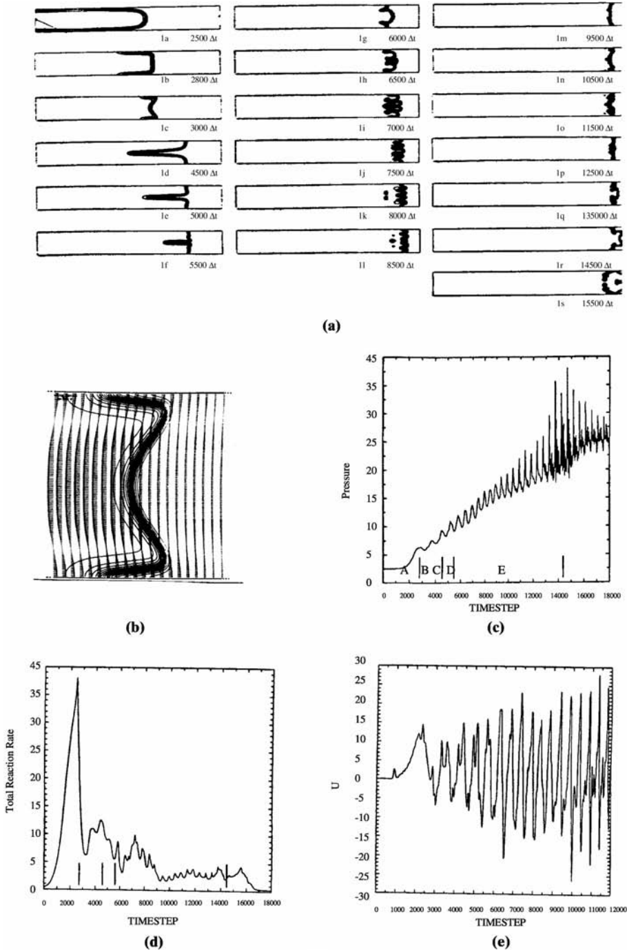
Figure 23.5.3.5 Unstable waves in flame propagation in a closed tube [Gonzales, 1996]. (a) Isolines of fuel mass fraction, 2500\Delta t \leq t \leq 15500\Delta t . (b) Flowfield in the vicinity of the flame t = 3000\Delta t . (c) Temporal evolution of pressure at the unburned end of the tube. (d) Temporal evolution of total reaction rate. (e) Temporal evolution of longitudinal velocity on the plane of symmetry at x/L = 0.9 .
