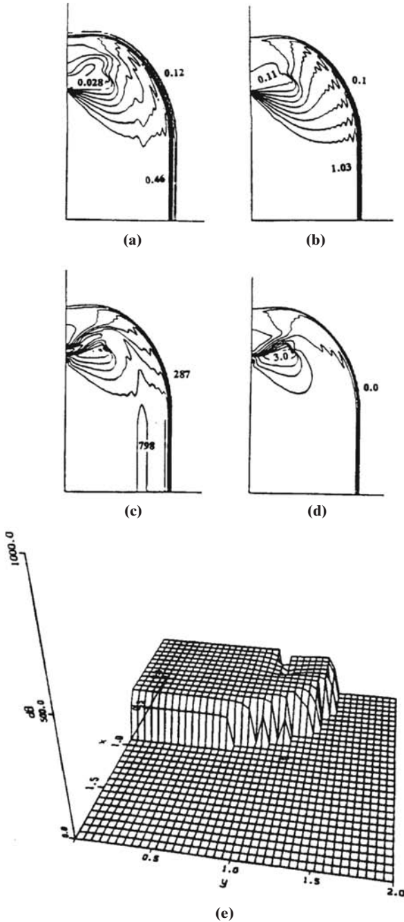
Figure 23.5.111 Noise level (dB) distribution and corresponding flowfields at t = 0.0012 sec. (a) Density distribution. (b) Pressure distribution. (c) Temperature distribution. (d) Mach number distribution. (e) Noise level (dB).
