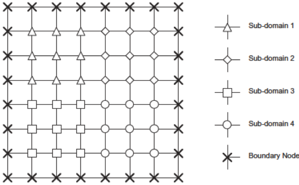
Figure 20.4.2.1 Multiple subdomains.
