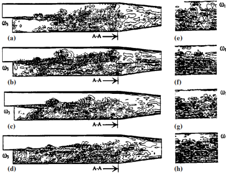
Figure 21.7.25 Instantaneous spanwise \bar{\omega}_3 and streamwise vorticity \bar{\omega}_1 contours normalized with the step height and inflow velocity in typical x1 - x2 and x2 - x3 planes: (a) \bar{\omega}_3 run A2, (b) \bar{\omega}_3 run B1, (c) \bar{\omega}_3 run B2, (d) \bar{\omega}_3 run C1, (e) \bar{\omega}_1 run A2, (f) \bar{\omega}_1 run B1, (g) \bar{\omega}_1 run B2, (h) \bar{\omega}_1 run C1 [Fureby, 1999].
