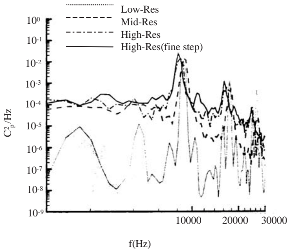
Figure 23.5.2.5 Spectra of pressure coefficient under vortex-generator plate for different grid resolutions M = 0.2 [Singer et al., 1999].
