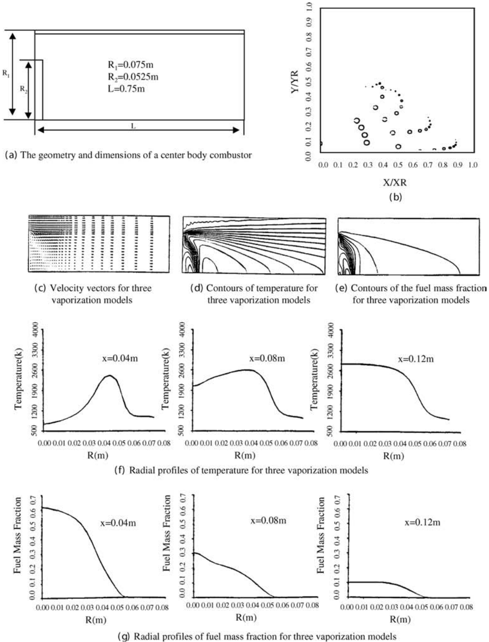
Figure 22.6.5.1 Spray combustion of center body combustor [Kim and Chung, 1990].
