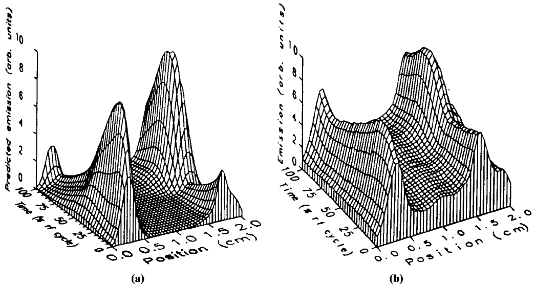
Figure 26.4.2.1 RF glow discharge [Gogolides and Swain, 1992]. (a) Predictions from a two-moment model for emission of the 750.4-nm argon line (1 torr, 2 cm spacing, 13.5 Mhz, and 0.14 \text{ W/cm}^2 ). (b) Experimentally measured emission.
