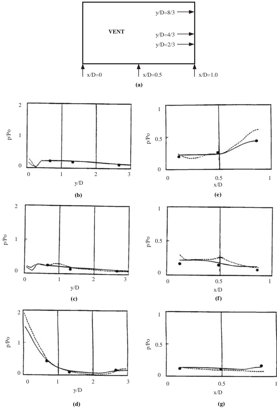
Figure 23.5.15 Comparison of pressure ratios ( P/P_0 ) with experiments, — TGM [Yoon and Chung, 1994], - - - - - TVD [Carofano, 1987], ● ● Experiment [Carofano, 1987]. (a) Locations of data. (b) X/D = 0.0 . (c) X/D = 0.5 . (d) X/D = 1.0 . (e) Y/D = 2/3 . (f) Y/D = 4/3 . (g) Y/D = 8/3 .
