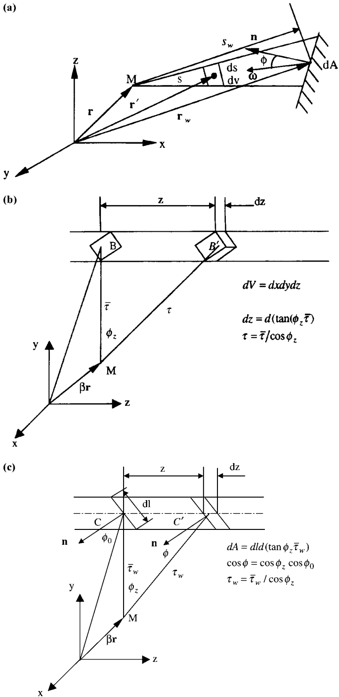
Figure 24.3.2 Three-dimensional heat flux integral formulation. (a) Radiation contribution of a surface element, dA , and a volume element, dv , to a point M in a direction \omega . (b) Geometry for volume integral. (c) Geometry for surface integral.
