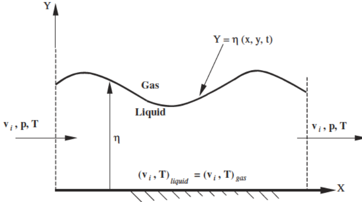
Figure 11.1.2 Free surface flow boundary conditions with variable temperatures as well as velocity and pressure between liquid and gas.
