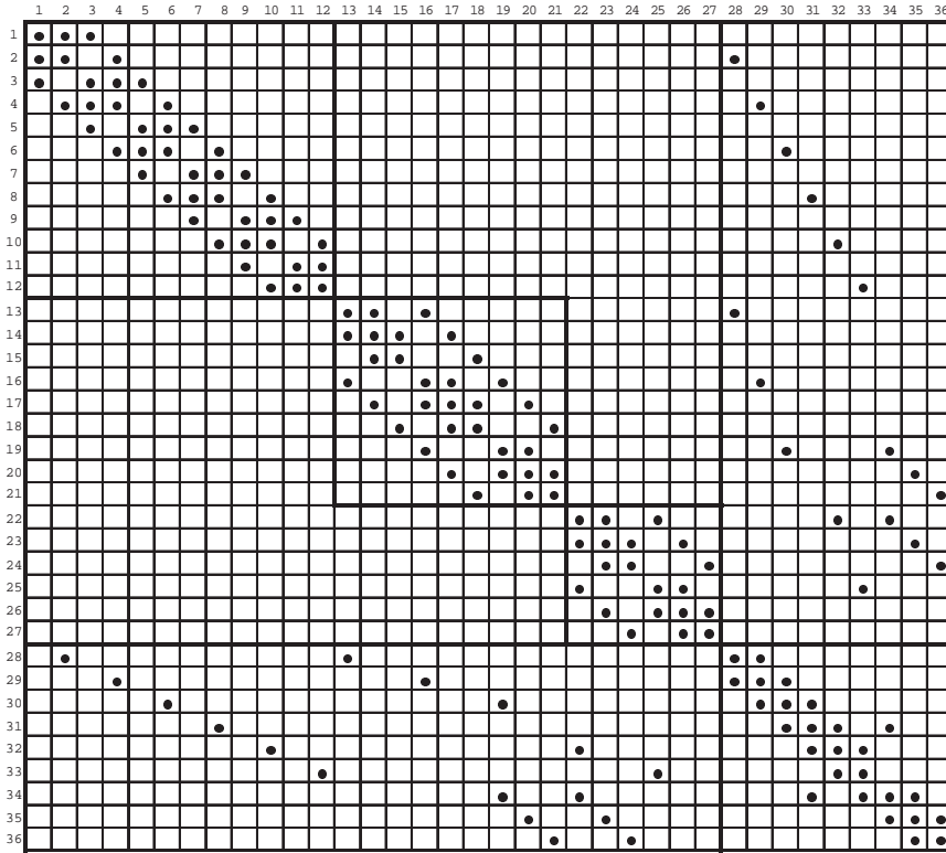
Figure 20.1.2 Global stiffness matrix, K_{aa}(27 \times 27) for Figure 20.1.1 with the subdomain stiffness matrices K_1(12 \times 12) , K_2(9 \times 9) , K_3(6 \times 6) , for \Omega_1 , \Omega_2 , \Omega_3 , respectively, and the boundary interface stiffness matrix, K_{bb}(9 \times 9) together with the interface-subdomain interaction stiffness matrices K_{ab}(27 \times 9) and K_{ba}(9 \times 27) .
