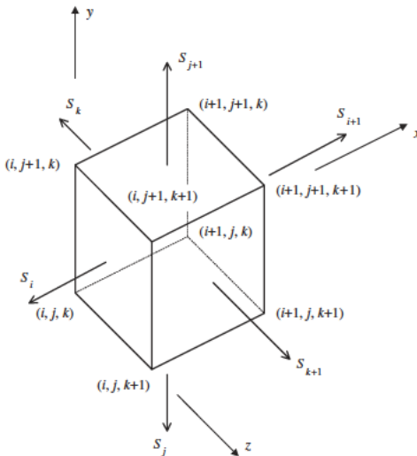
Figure 7.3.6 Three-dimensional discretization.
