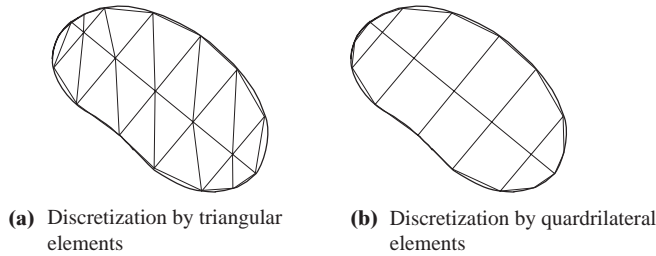
Figure 9.1.1 Finite element discretization of a two-dimensional domain.
