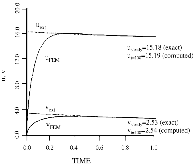
Figure 10.4.2.2 Convergence history of u and v ( v = 1.0 , \Delta t = 0.01 , x = 4.5 and y = 0.75 ).
