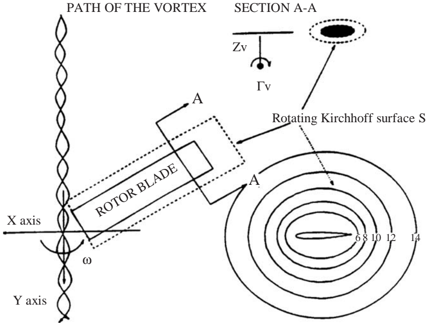
Figure 23.5.1.6 Hover parallel blade-vortex interaction and rotating Kirchhoff surface S [Xue and Lyrintzis, 1994].
