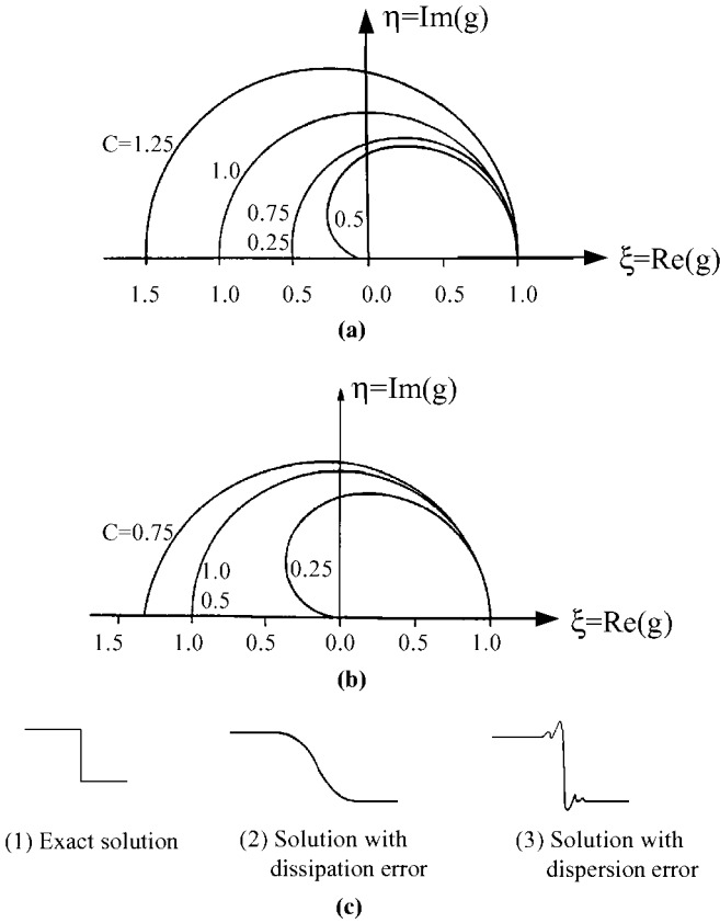
Figure 4.3.2 Dissipation and dispersion errors compared to exact solution. (a) Dissipation error (amplification factor modulus |g| ). (b) Dispersion error (relative phase error, \Phi/\Phi ). (c) Comparison of exact solution with dissipation error and dispersion error for shock tube problem.
