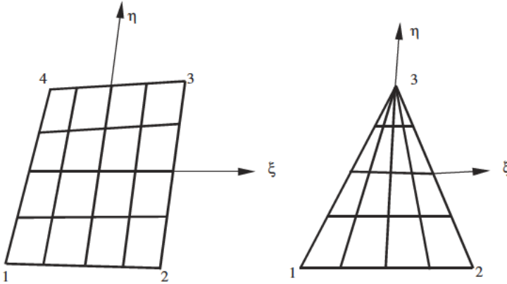
Figure E9.3.5 Collapsing a quadrilateral element into a triangle. Gaussian quadrature integration can be performed on the triangle as modified from the quadrilateral.
