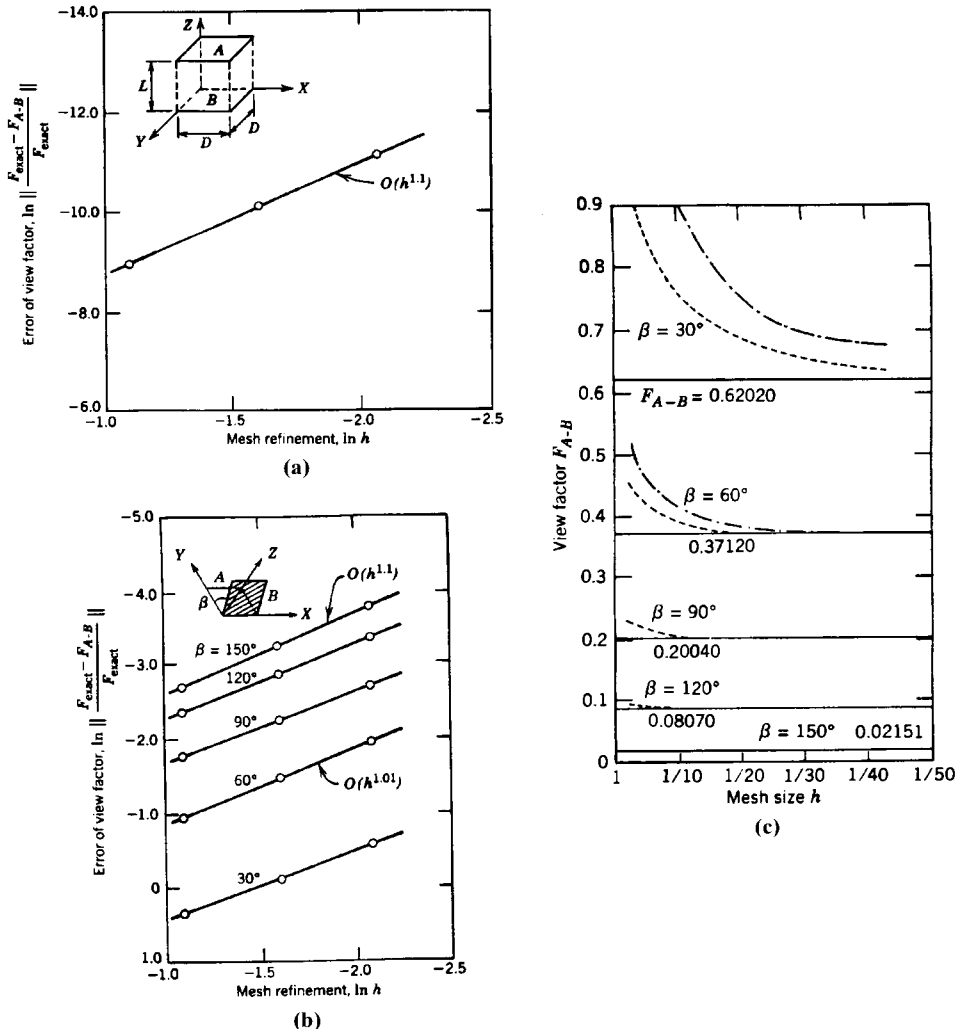
Figure 24.4.1.1 View factor calculations, convergence studies. (a) Convergence curve of view factor error vs. mesh size for two parallel 1 \times 1 square planes, one unit apart. (b) Convergence curve of view factor error vs. mesh size for two intersecting 1 \times 1 square planes at angle of 30^\circ, 60^\circ, 90^\circ, 120^\circ, 150^\circ . (c) View factors vs. mesh size, intersecting planes. (—) exact solution; (—●—) two-point Gaussian quadrature; (-----) six-point Gaussian quadrature.
