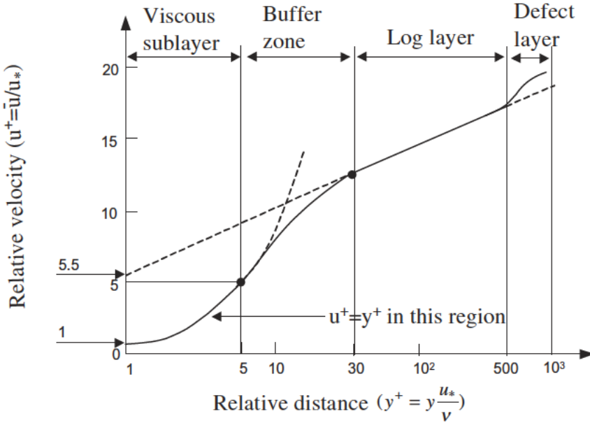
Figure 21.3.1 Two-dimensional turbulent boundary layer velocity profile showing various layers in terms of shear velocity u_* = \sqrt{\tau/\rho} .
