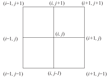
Figure 3.4.1 Two-dimensional mesh.
