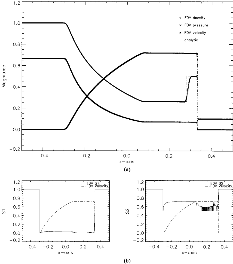
Figure 27.3.4.1 Relativistic shock tube analyzed by the FDV theory, 1,600 nodes, CFL = 0.18, \alpha = 0.001 , and \eta = 0.25 [Richardson, 2000]. (a) Density, pressure, and velocity distributions. (b) Calculate values of convection variation parameters ( s_1, s_2 ).
