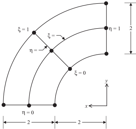
Figure E17.1.6 Quarter-circle disk with TIF method.
