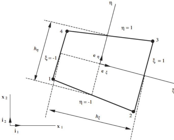
Figure 11.3.3 Four node isoparametric element; e_\xi and e_\eta are the unit vectors along the \xi and \eta axes, respectively.
