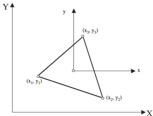
Figure 9.3.1 Cartesian coordinate triangular element.
