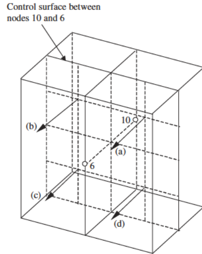
Figure 7.4.1 Control surface [normal vectors (a), (b), (c), (d)] between nodes 10 and 6 of Figure 7.3.1.
