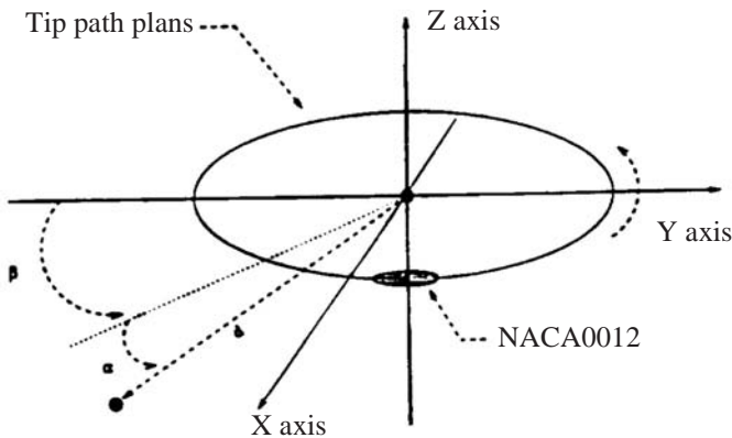
Figure 23.5.1.7 Observer's position for a rotating blade [Xue and Lyrintzis, 1994].
