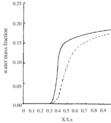
(i) Water distribution
