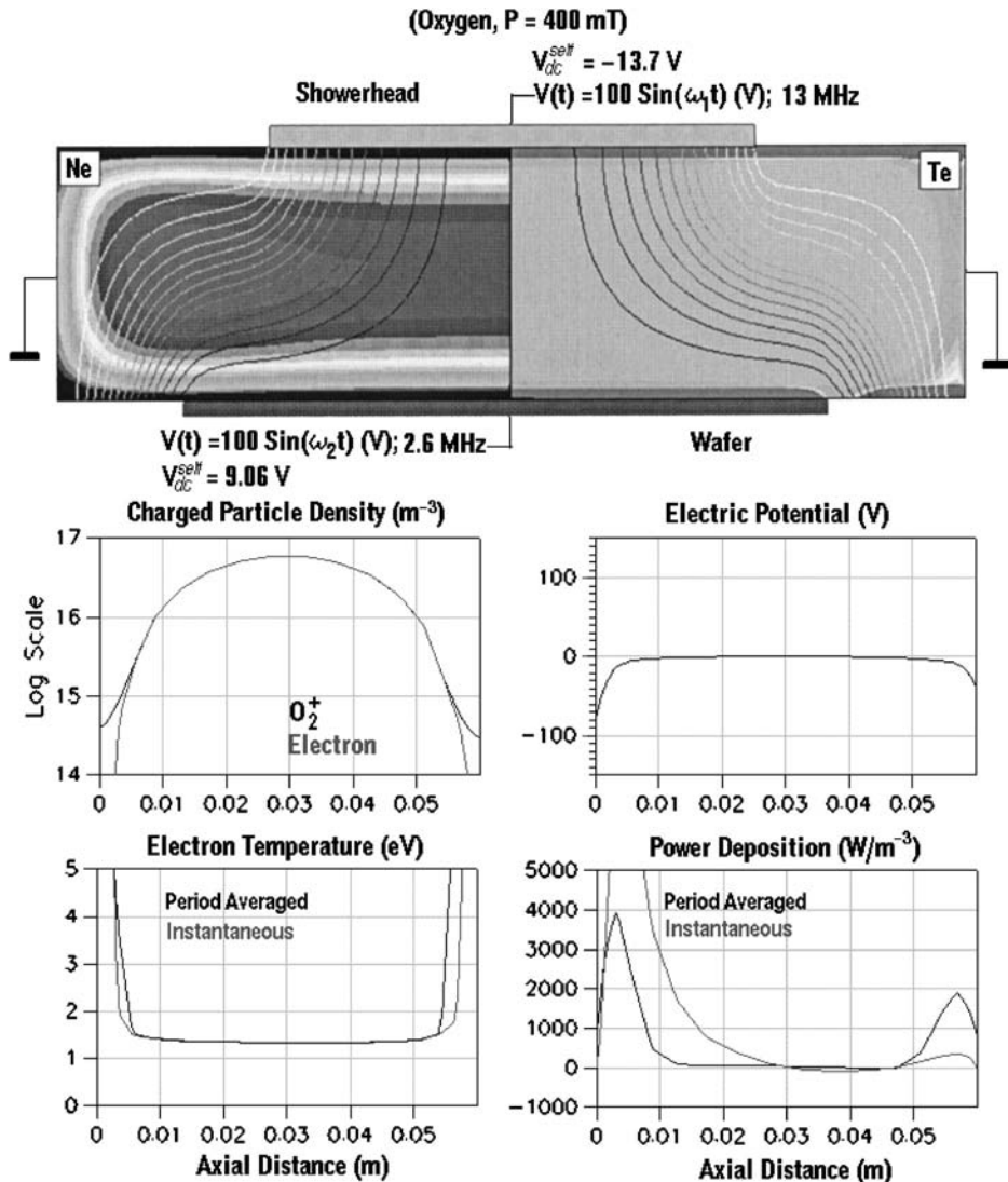
Figure 26.4.2.3 Dual-frequency capacitively coupled plasma [Courtesy of CFDRC].
