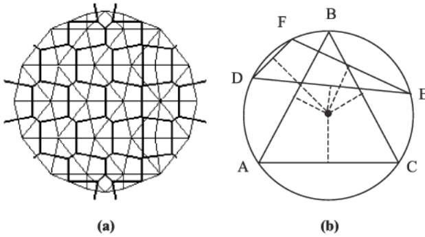
Figure 18.1 Delaunay triangulation with Voronoi polygon, and triangle's circumcircle. (a) Delaunay triangulation and Voronoi polygon. (b) Triangle and its circumcircle.
