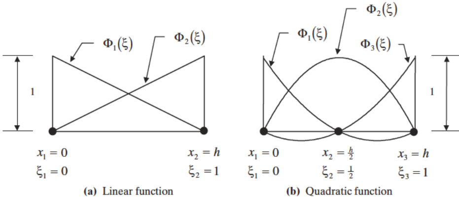
Figure 17.1.1 Lagrange polynomials.
