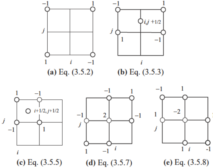
Figure 3.5.1 Mixed derivatives.
