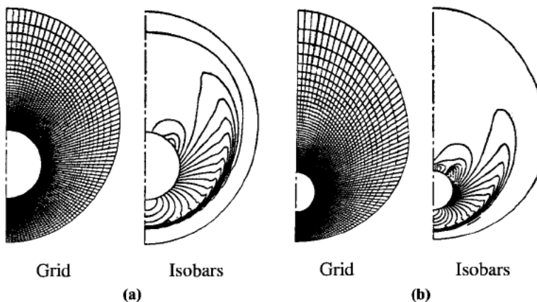
Figure 7.5.1 FVM/FDM solutions of Euler equations for flows over a circular cone [Siclari and Jameson, 1989]. (a) Euler grid and computed isobars for a 20^\circ circular cone at M_\infty = 2.0 , \alpha = 25^\circ . (b) Euler grid and computed isobars for a 10^\circ circular cone at M_\infty = 2.0 , \alpha = 25^\circ .
