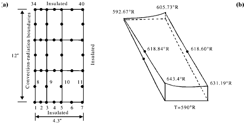
Figure 24.4.1.2 Heat conduction with convection and radiation boundaries. (a) 3 \times 3 quadratic elements (40 nodes), Example 24.2.2 case 1. (b) Temperature distribution, Example 24.2.2 case 1.
