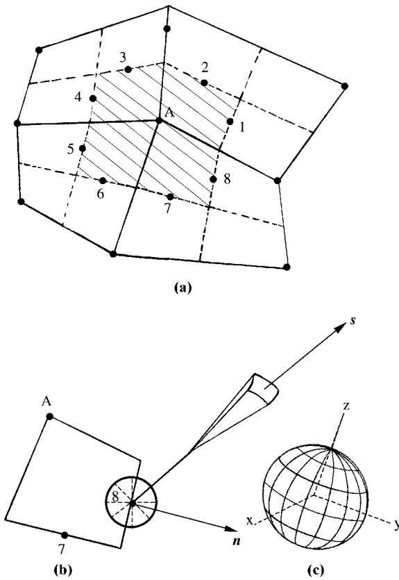
Figure 24.2.4 Finite volume representation via finite elements for control boundary surfaces and control angle directions. (a) Finite volume representation at A with boundary nodes, 1-8. (b) Designation of \mathbf{n} and \mathbf{s} at boundary node 8. (c) Subdivision of directional solid angles at boundary node 8.
