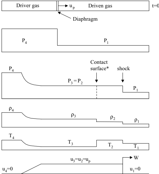
Figure 6.5.1 Mechanism of shock wave discontinuities as related to s_a in terms of the changes of Mach number with respect to the velocity and square root of pressure, density, or temperature, s_a = f(u/\sqrt{p/\rho}) = f(u/\sqrt{RT}) = f(M) .
