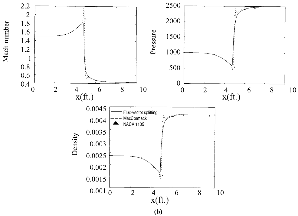
Figure 6.8.1.1 Quasi-one-dimensional supersonic nozzle flow. (a) Case 1 supersonic inflow-supersonic outflow. (b) Case 2 supersonic inflow-subsonic outflow.
