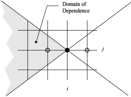
Figure 6.1.1 Region of dependence.
