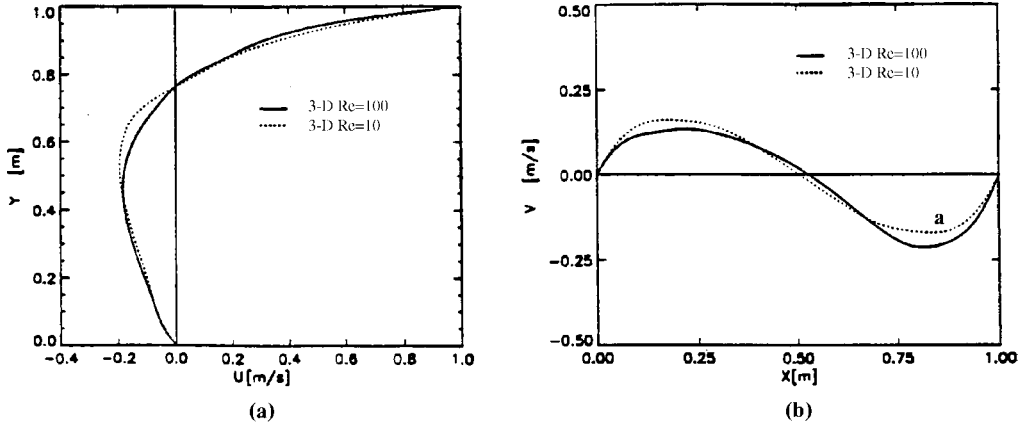
Figure 12.3.5 Velocity profile on the 3-D cavity. (a) Vertical centerline. (b) X-horizontal centerline.
