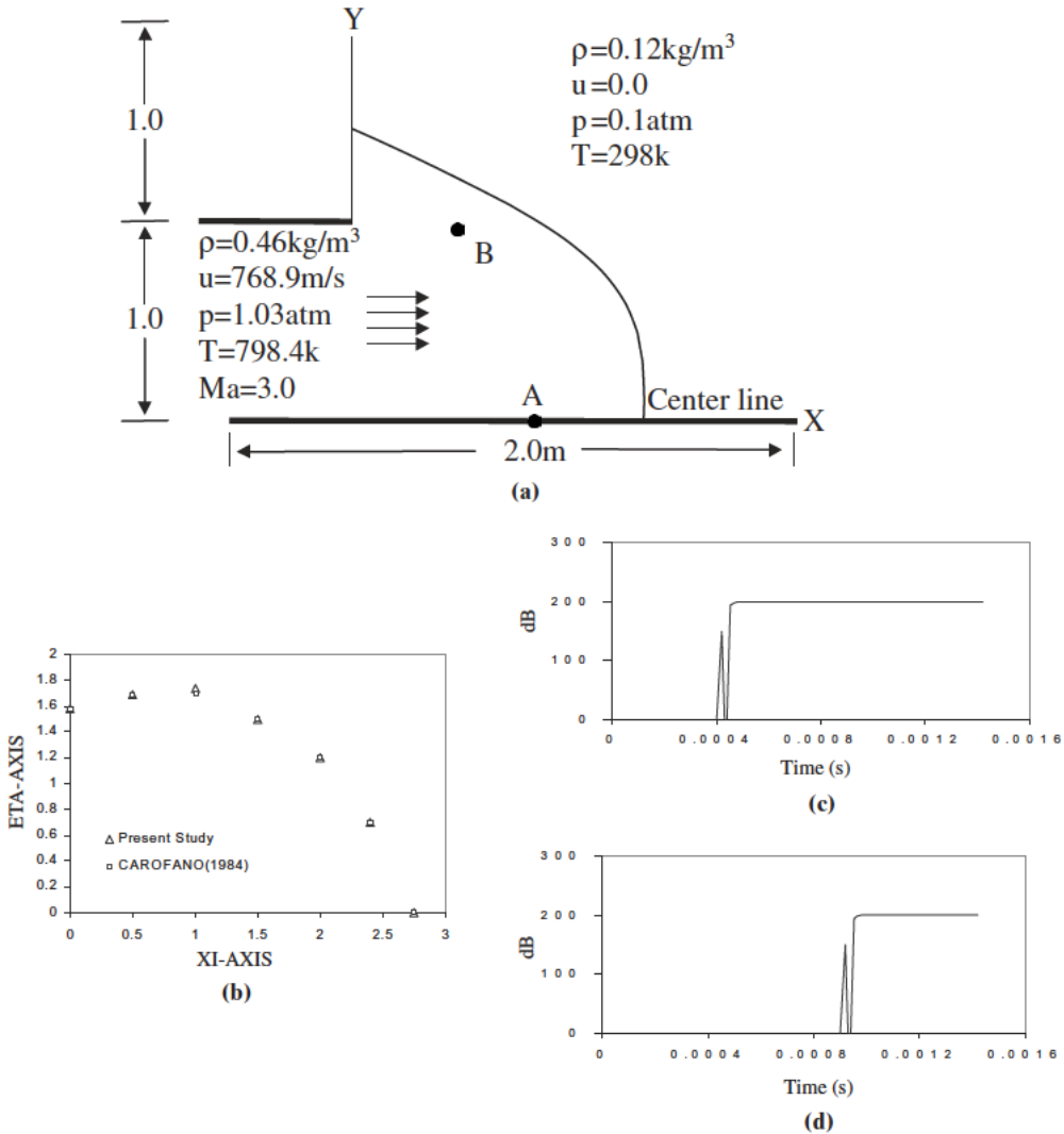
Figure 23.5.110 Geometry, initial and boundary conditions for the rocket nozzle exhaust. (a) Geometry and initial and boundary condition. (b) Shock locations at t = 0.0012 \text{ sec} . (c) Noise level at point A. (d) Noise level at point B.
