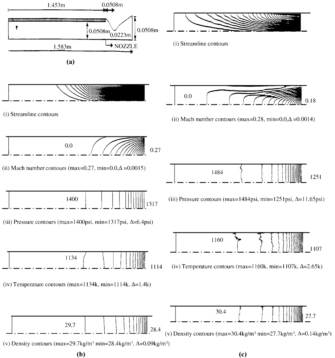
Figure 23.5.3.1 State flowfield for side-burning rocket motor, burning surface boundary conditions: \rho = 29.7 \text{ kg/m}^3 , V = 1.22 \text{ m/s} , T = 1134 \text{ K} , P = 1400 \text{ psi} , Mach no. = 0.0018, laminar calculations [Yoon and Chung, 1994]. (a) Geometry. (b) 0% disturbance. (c) 6% disturbance.
